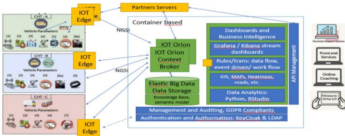
Figure 3. The Panacea Platform
